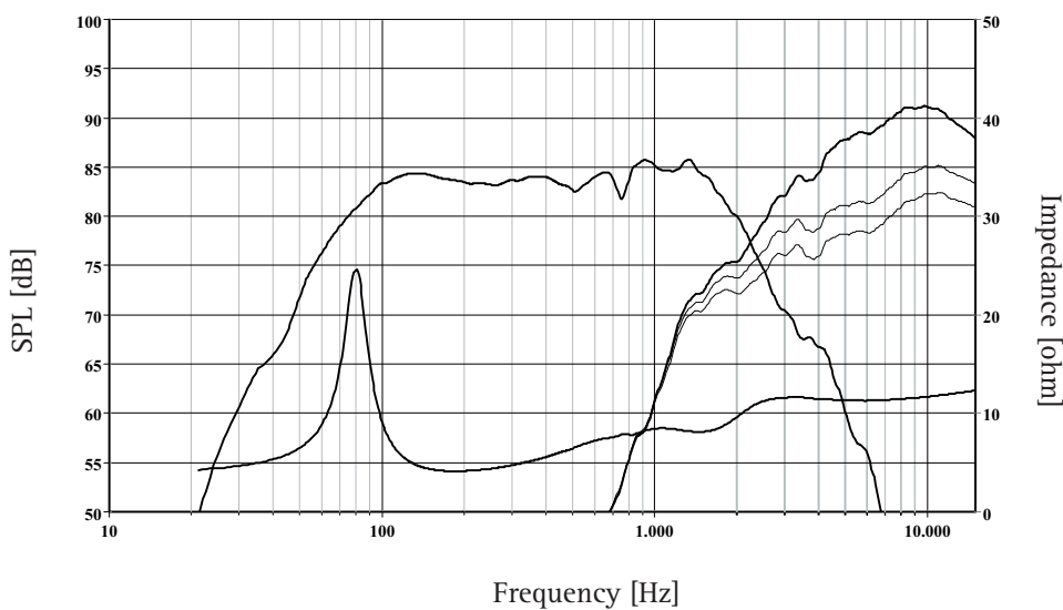
The frequency responses above show measured free field sound pressure for the RW165/1 and RT27F with cross over. The graph is also showing the tweeter adjustments available in the crossover. Input 2.83 V RMS , microphone distance 0.5m, normalized to SPL 1m. The impedance is measured using a 2V sine signal.
