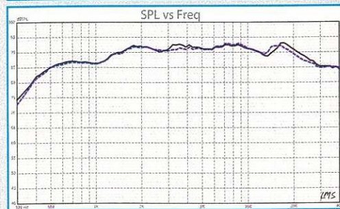
FIGURE 5: D3004/602010 two-sample SPL comparison.
