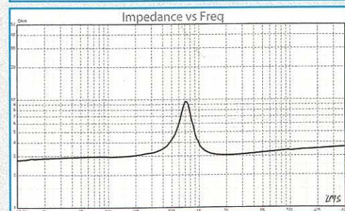
FIGURE 9: ScanSpeak D3004/602010 free-air impedance plot.
