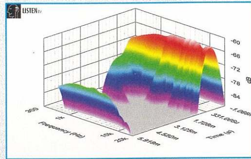
FIGURE 7: D3004/602010 SoundCheck STFT surface intensity plot.
