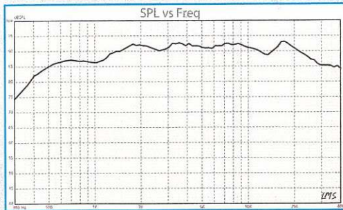
FIGURE 2: D3004/602010 on-axis response.
