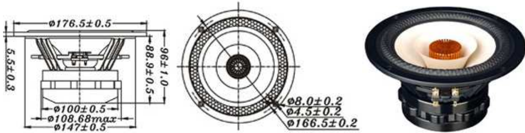
6.5" PAPER FULL RANGE
